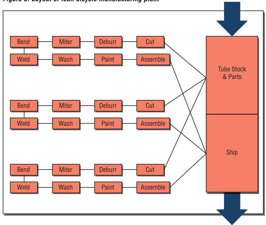
Figure 3: Layout of lean bicycle manufacturing plant
