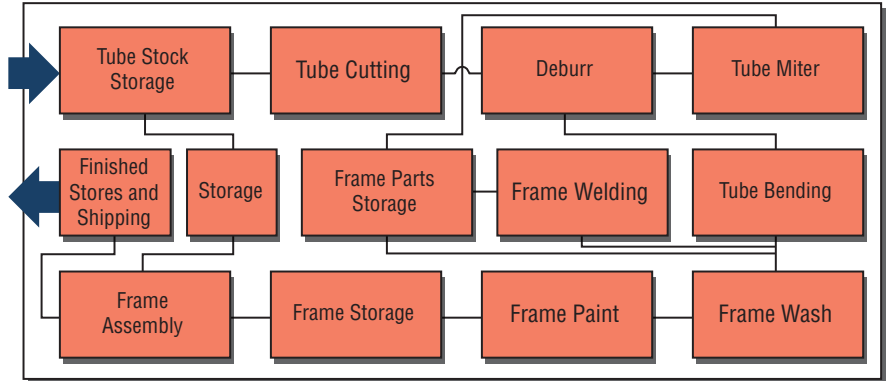
Figure 2: Layout of traditional bike manufacturing plant
